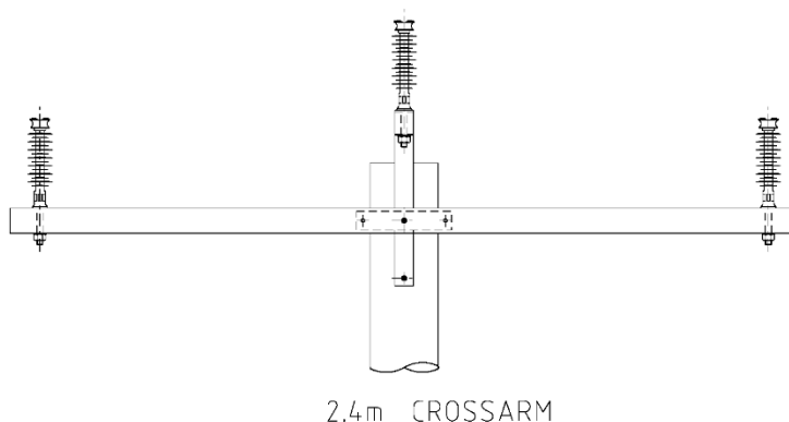
Figure 2-1: Typical arrangement at intermediate locations
